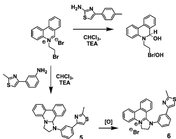
Scheme 3 Comparison of reaction path and reaction outcome between the amine isomers, 2-methyl-4-(3-aminophenyl)thiazole and 2-amino-4-( p -tolyl)thiazole.
