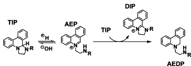
Scheme 2 Relationship between the TIP, DIP, AEP and AEDP structures by way of pH control.
