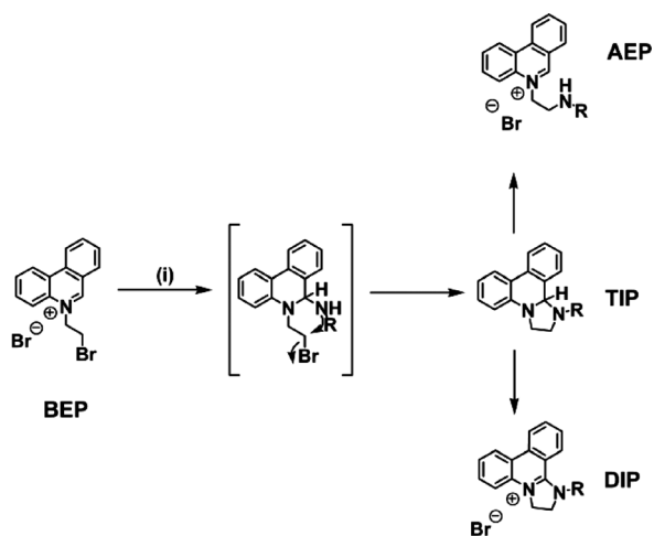
Scheme 1 Synthetic outline for the preparation of the TIP, DIP and AEP heterocycles (i) \text{NH}_2\text{R} (1 eq.) and triethylamine (3 eq.) in chloroform.
